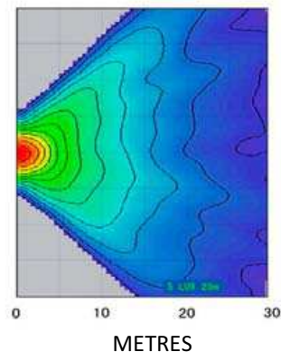
FLOOD BEAM PATTERN
